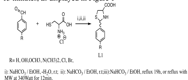
Figure 1: General diagram showing the synthesis of thiazolidine (thiazolidine-4-carboxylic acid) and its derivatives.
