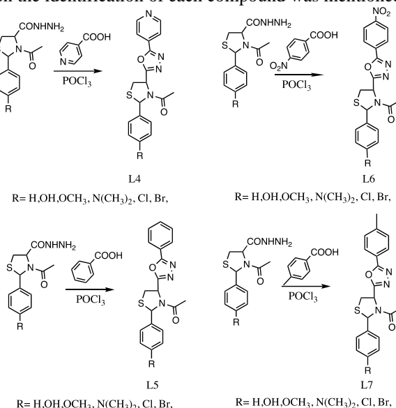
Figure 3: Synthesis diagram of L4-L7 compounds
