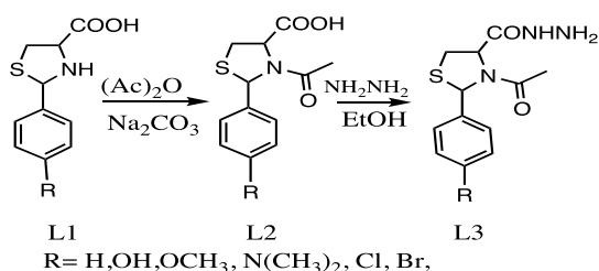
Figure 2: L2 and L3 synthesis diagram.
