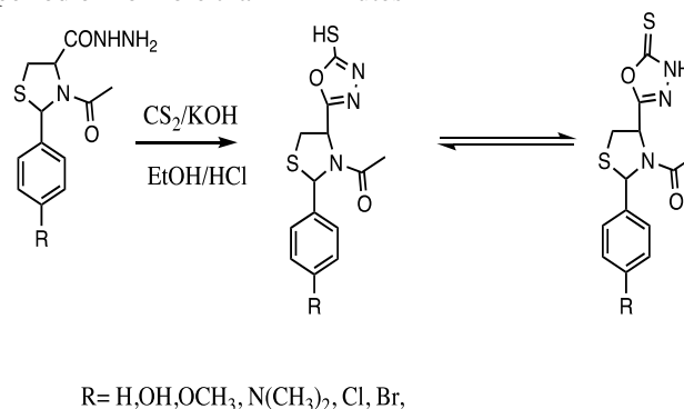
Figure 4: L8. synthesis diagram
